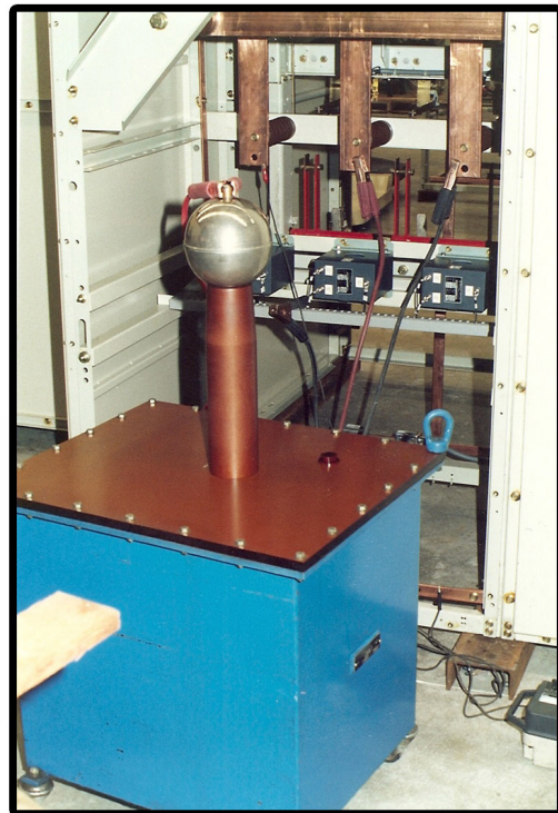
22kV Switchboard > QA Highpot Testing
