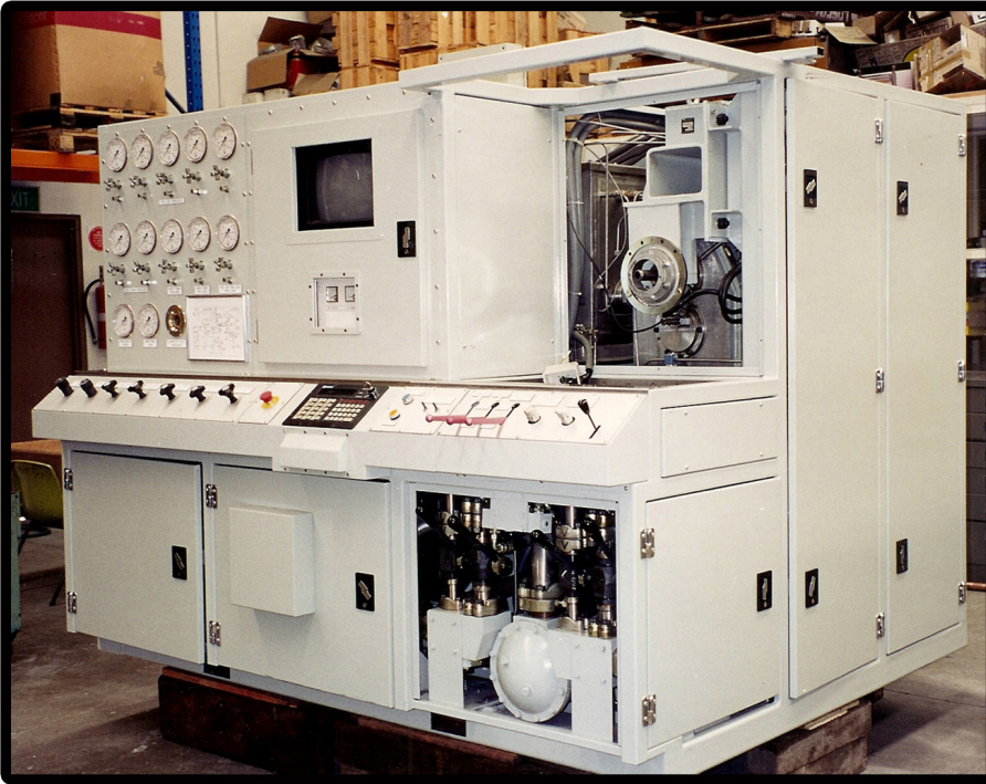
Aircraft Test Station MH624 Rotating Components
