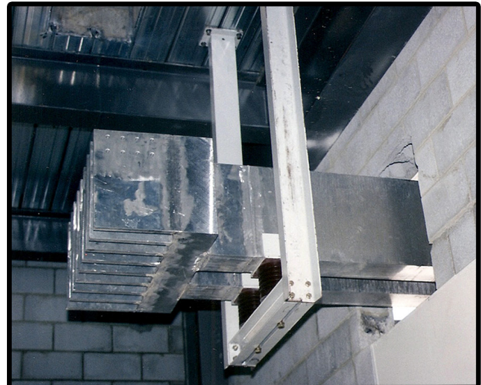
DC Rectifier 117VDC, 56kA Two 400x 150mm Al Busbars
