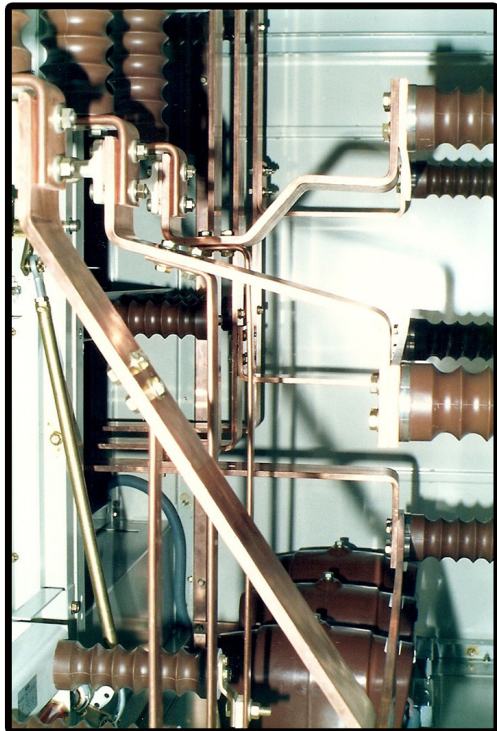
< 22kV Switchboard Internal Busbars
