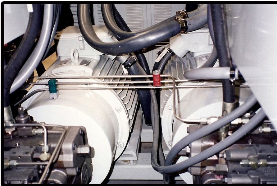
Aircraft Test Station MH624 Main Pumps - 2x 70USGPM @ 5000psi
